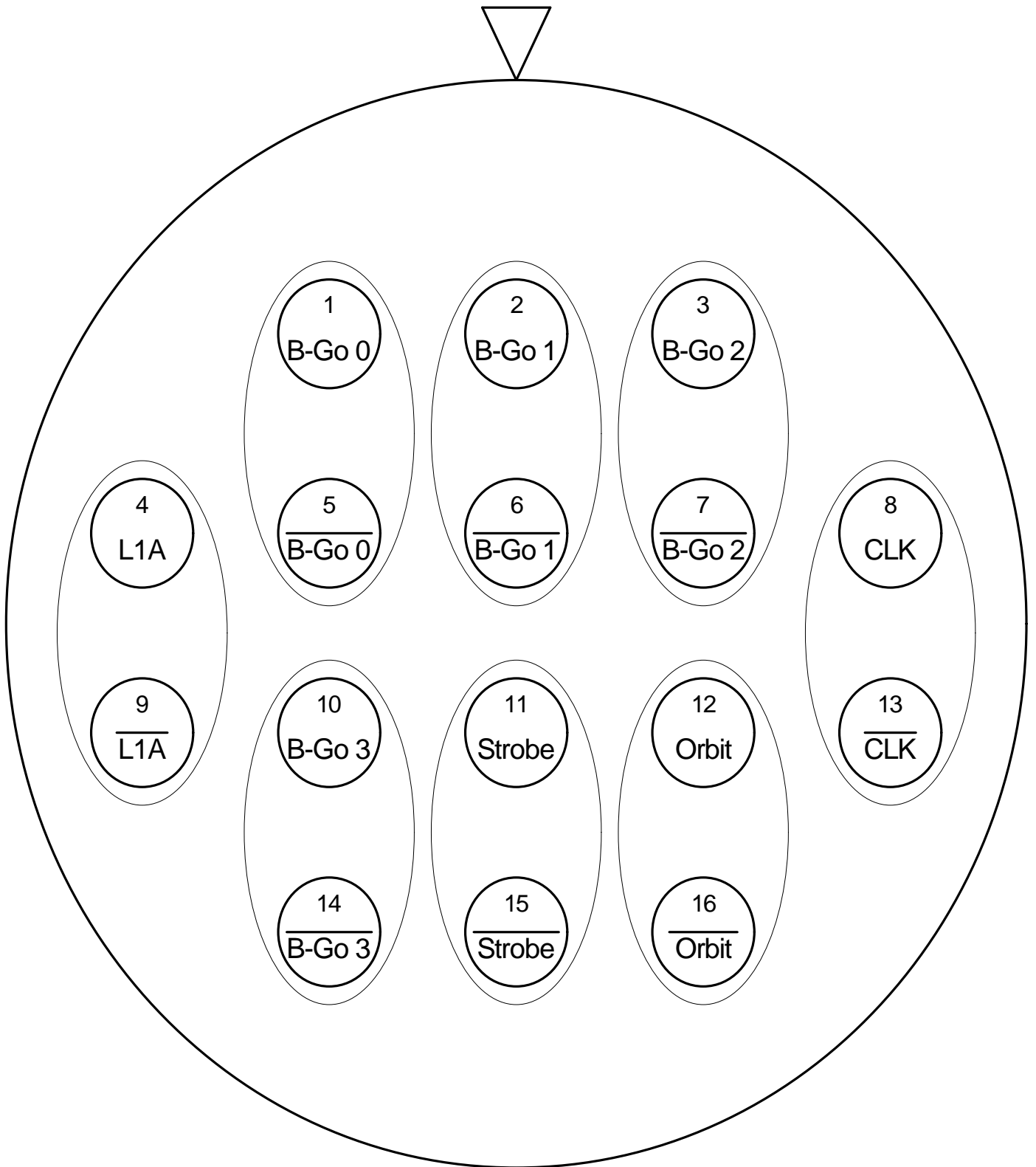
RECEPTACLE DIP POST CONFIGURATION
